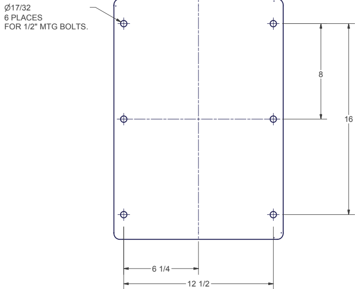
BACK VIEW
