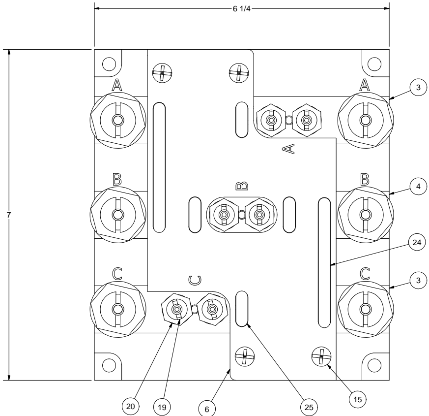
FRONT VIEW TERMINAL BASE ASSEMBLY
