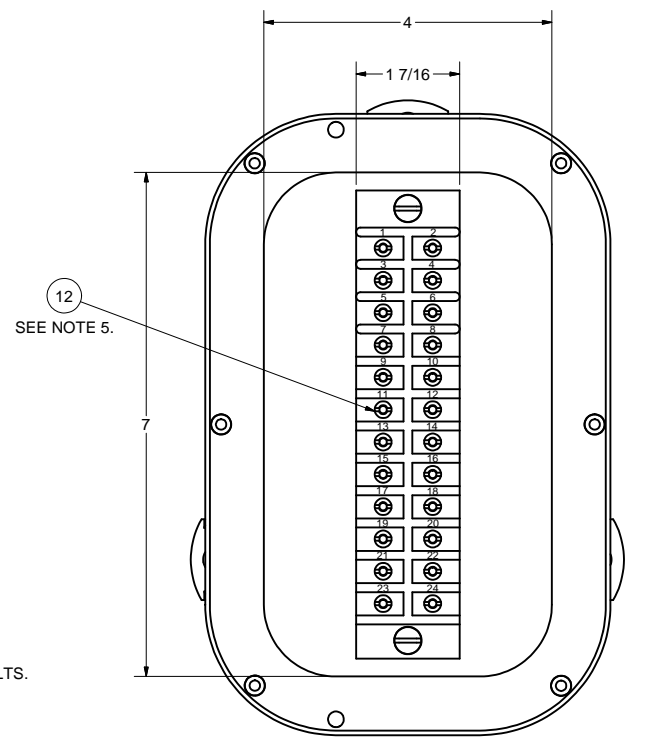
FRONT VIEW LESS COVER
